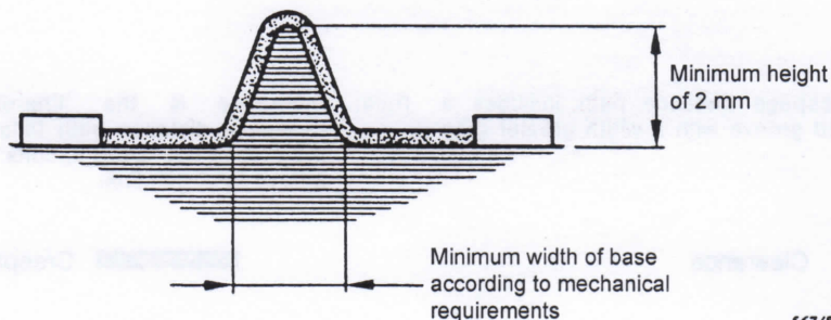
Figure F.1 – Measurement of ribs
